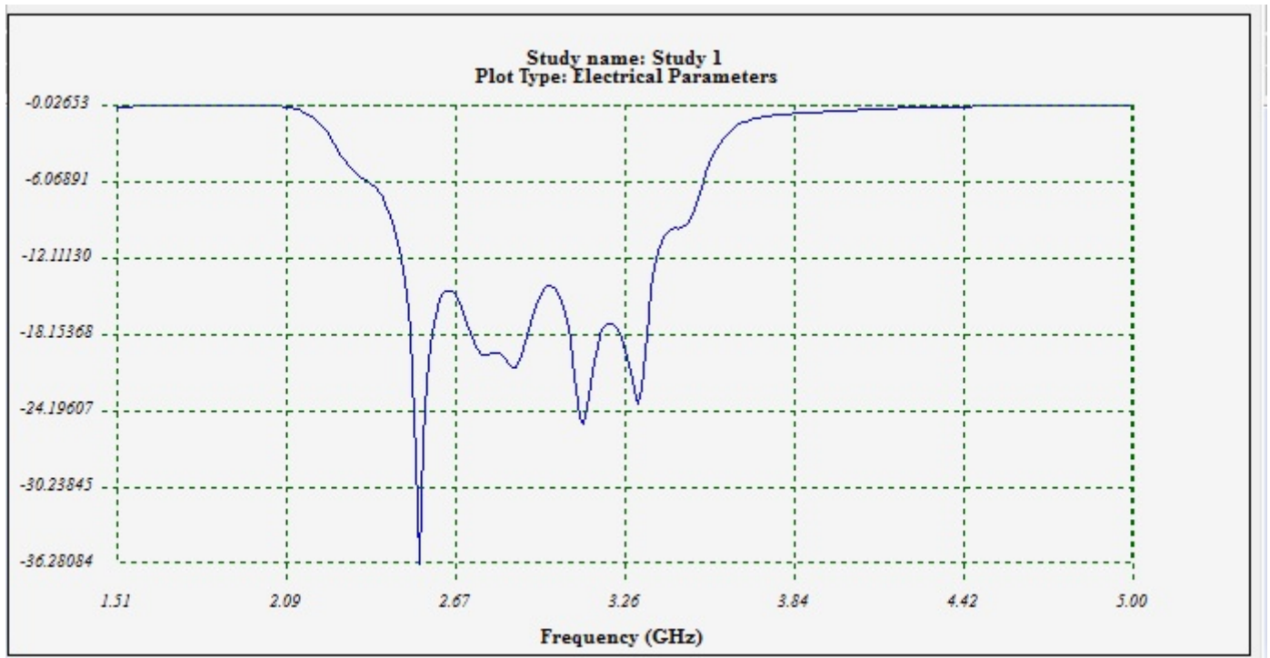
Figure 4 - Reflection coefficient at the antenna's port
